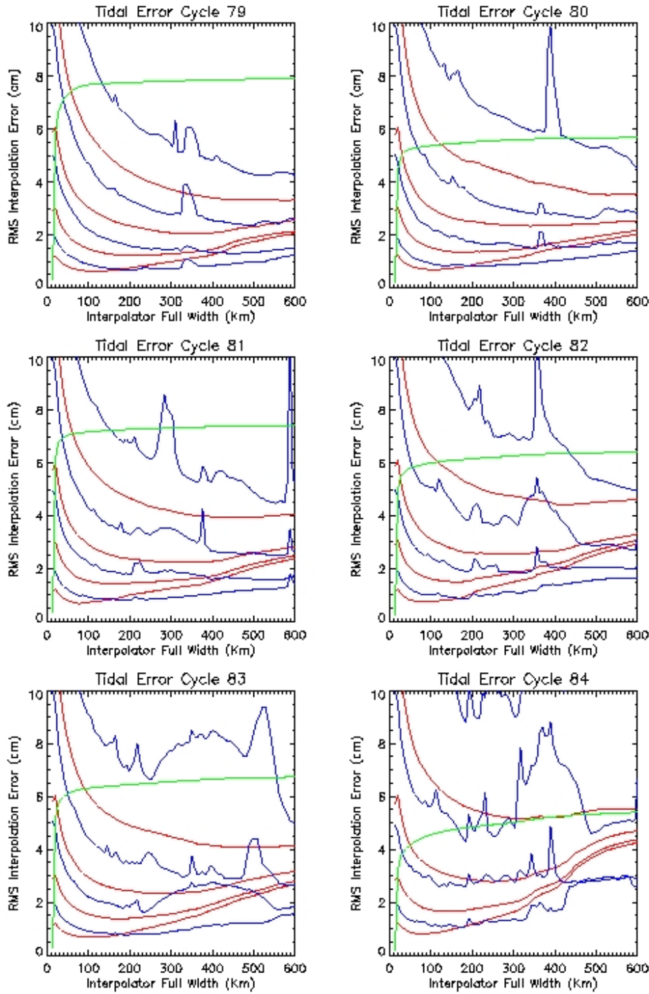
Fig. 4.18: Interpolation of Residual Tidal Signal. Comparison of RMS linear interpolation error (red) with RMS quadratic interpolation error (blue). Number of successful interpolations is shown in green. RMS random noise of 2cm, 5cm, 10cm, and 20cm added.
