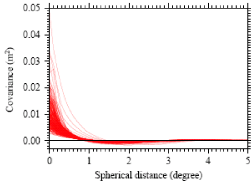
Fig. 1.25: Error covariance functions along the meridian of 15^\circ computed from \varphi=64^\circ to \varphi=90^\circ , with equidistance 0.1^\circ .
