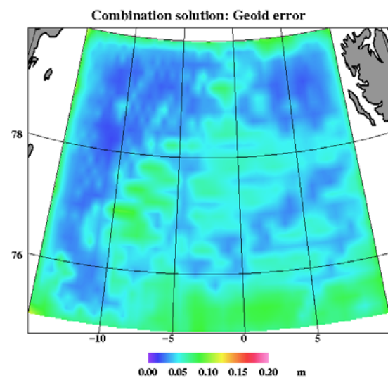
Fig. 1.42: Estimated errors of geoid based on MSS and gravity data combined.
