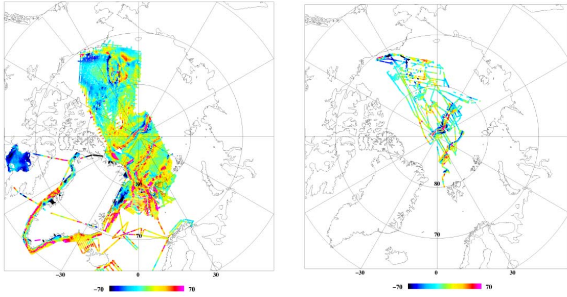
Fig. 1.1: Arctic Gravity Project coverage of NRL and DNSC high-quality airborne gravity data (left); SCICEX submarine data 1993-98 (right). Color scale is free-air gravity anomalies in mGal ( 10^{-5} \text{ m/s}^2 )
