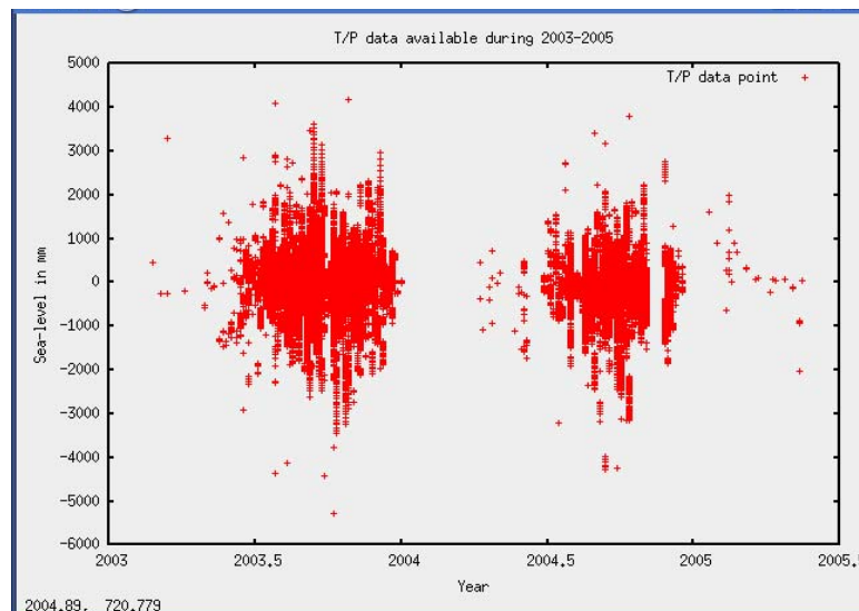
Fig. 3.26: T/P data available between 2003-2005 near Churchill. Winter month are not covered by observations.
