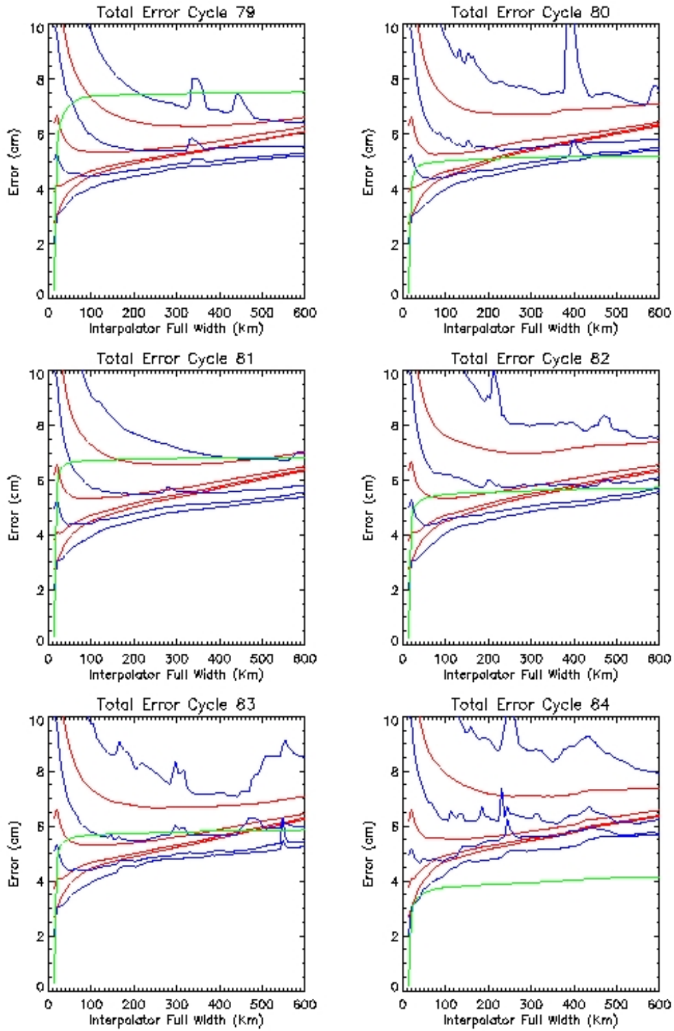
Fig. 4.27: Interpolation of Total Error Signal with Correlation Length = 11.10 km and Sigma = 5 cm. Comparison of RMS linear interpolation error (red) with RMS quadratic interpolation error (blue). Number of successful interpolations is shown in green. RMS random noise of 2cm, 5cm, 10cm, and 20cm added.
