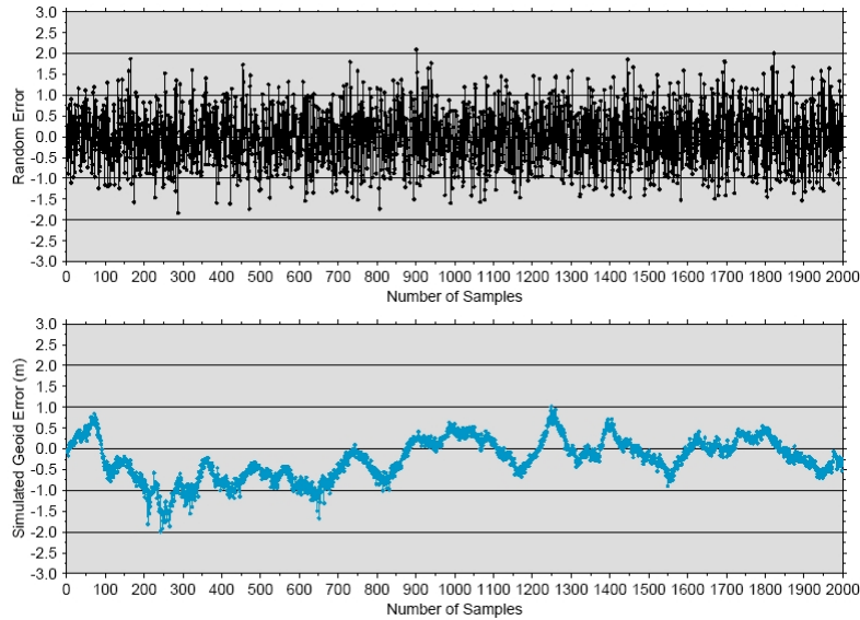
Fig. 4.9: (a) A portion of an initial Gaussian random number sequence which has a mean of 0 cm and a standard deviation of 66 cm. (b) The re-sequenced random number series representing a profile of geoid error with a standard deviation of 66 cm, correlation length of 0.47^\circ , and a covariance function that coincided with computed values.
