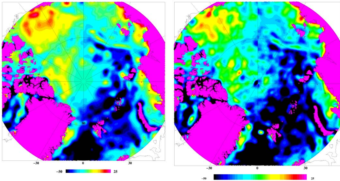
Fig. 3.29: Low-pass filtered MDT from remote sensing: MDT from MSS with ArcGP geoid (left) and EIGEN-GL4C (right). Unit: cm.
