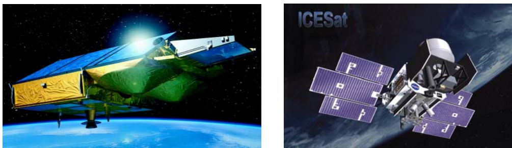
Fig. 2. CryoSat-2 (left) and ICESat (right) – complementary interferometric radar and laser missions, both with the possibility to map sea ice freeboard in the central Arctic Ocean. The results of the present study will hopefully add information on the accuracy of the freeboard recovery for both missions (ESA and NASA illustrations).
