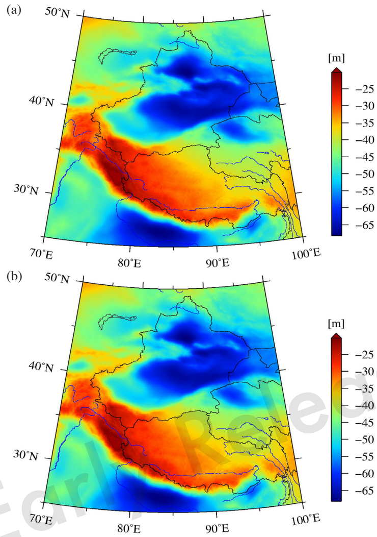
Fig. 9. (a) 5' x 5' EGM2008 regional geoid; (b) 5' x 5' calculated regional geoid.
