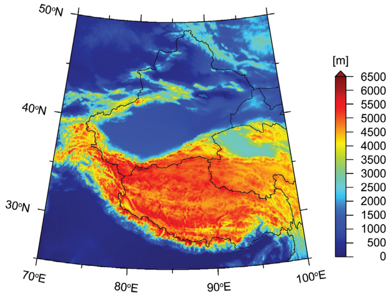
Fig. 4. A 5' \times 5' topography of the area of interest (AOI) determined by DTM2006.0.
