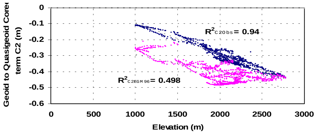
Fig-4. Relationship of Elevation with geoid-quasigeoid correction C2 term from observed gravity data and EGM96 model gravity in the Kalat area
