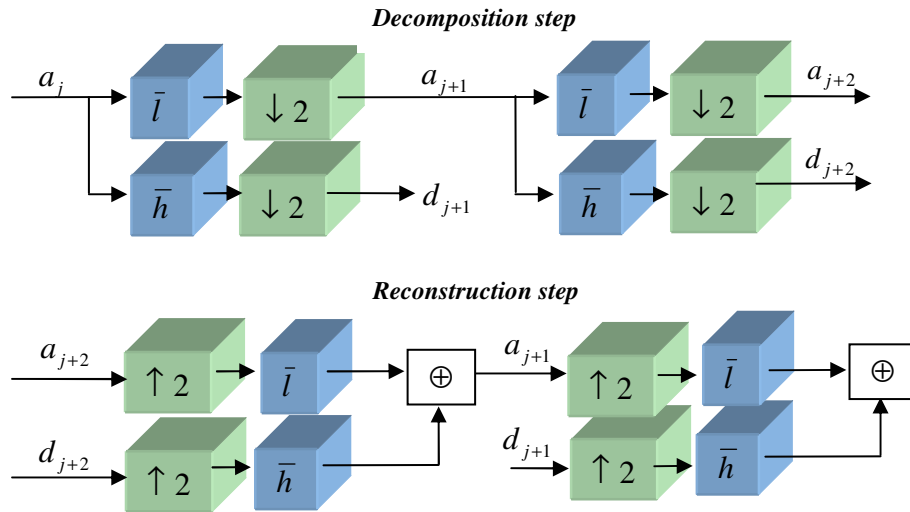
Fig.1 Decomposition and reconstruction steps in the wavelet-based multiresolution analysis (MRA).
