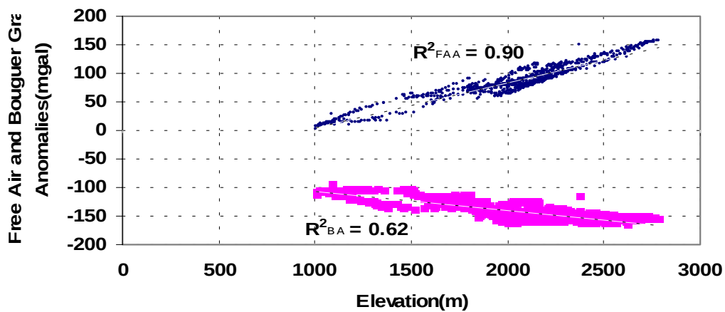
Fig-2. Relationship of Elevation with Free Air and Bouguer gravity Anomalies in Kalat Area
