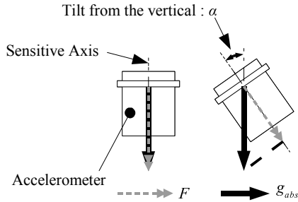
Fig. 1 Tilt of accelerometer sensitive axis
