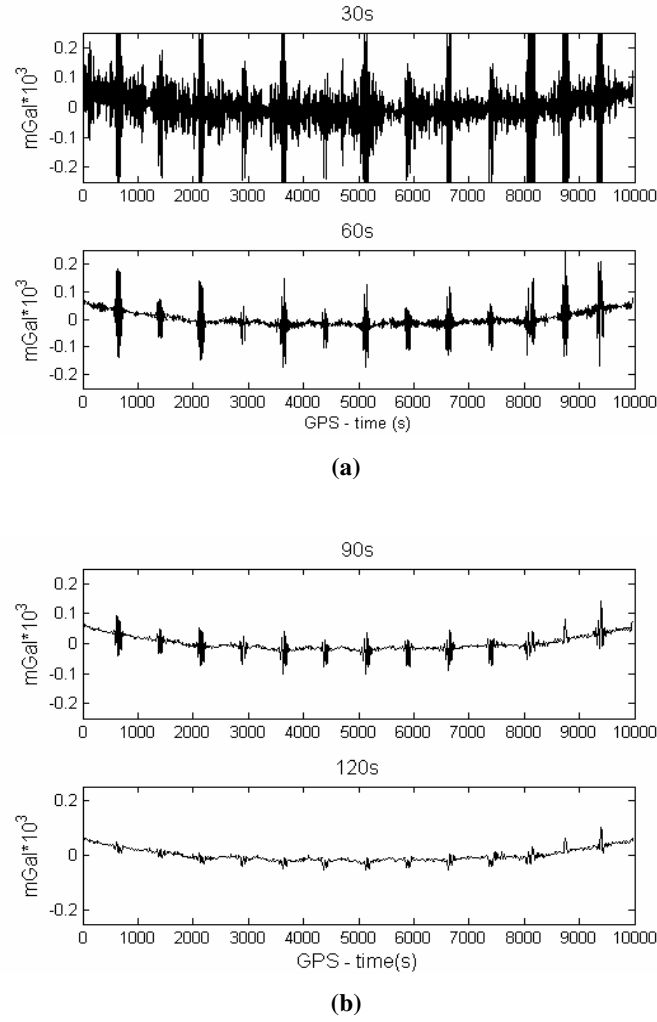
Fig. 7 (a) Difference between reference data and 30s, and 60s low pass filter output. (b) Difference between reference data and 90s, and 120s low pass filter output.
