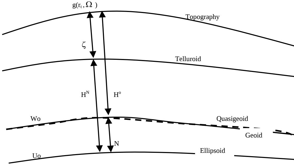
Figure-1: The geoid undulation( N ), Orthometric heights ( H ), Height Anomaly ( \zeta ) and Normal heights ( H^N )
