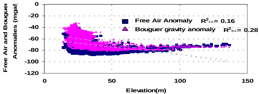
Fig-3. Relationship of Elevation with Free Air and Bouguer gravity Anomalies in Dadu Area
